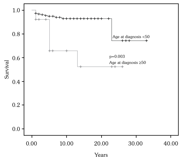
Figure 1. Survival by age of systemic lupus erythematosus diagnosis (Kaplan-Meier method).
